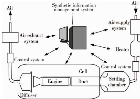
Fig. 2 Sketch map of the ATF
