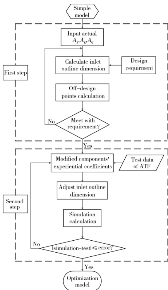
Fig. 3 Flow chart of the model optimization
